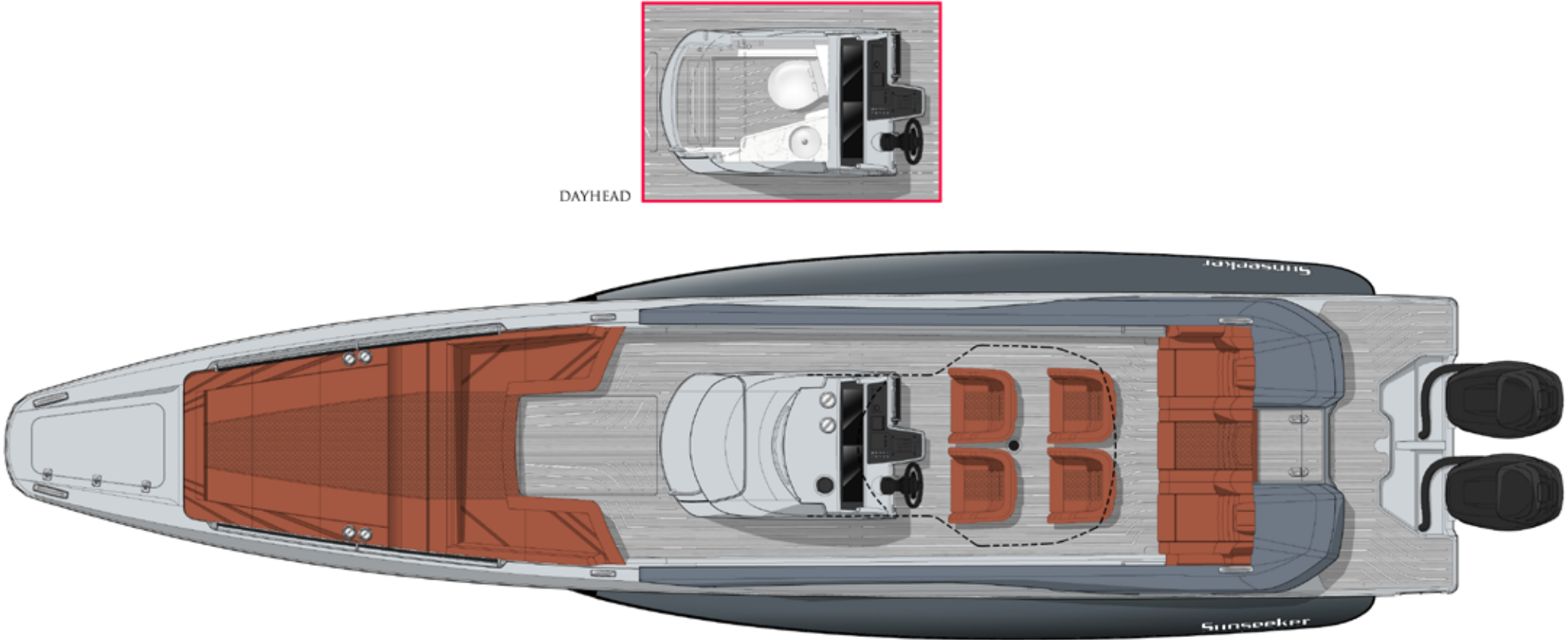
EXTERIOR PLAN
